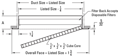
CC5F-6 - Return Grille - Lay in T-Bar
